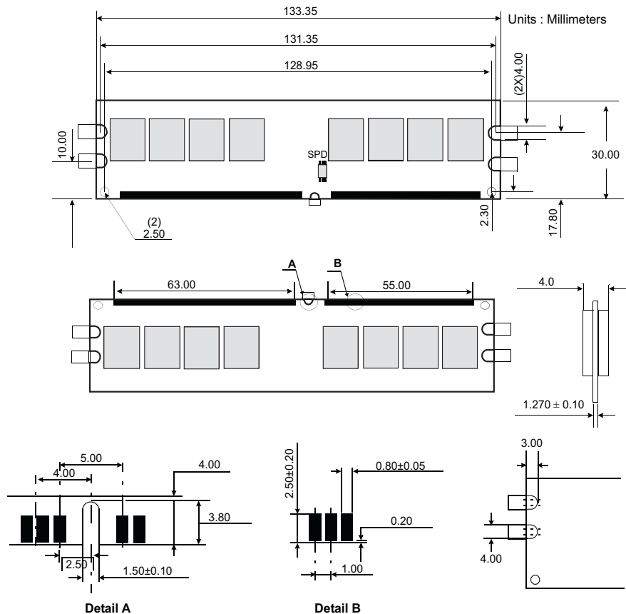
Figure 1: KVR400D2N3/1G 240-Pin DIMM
